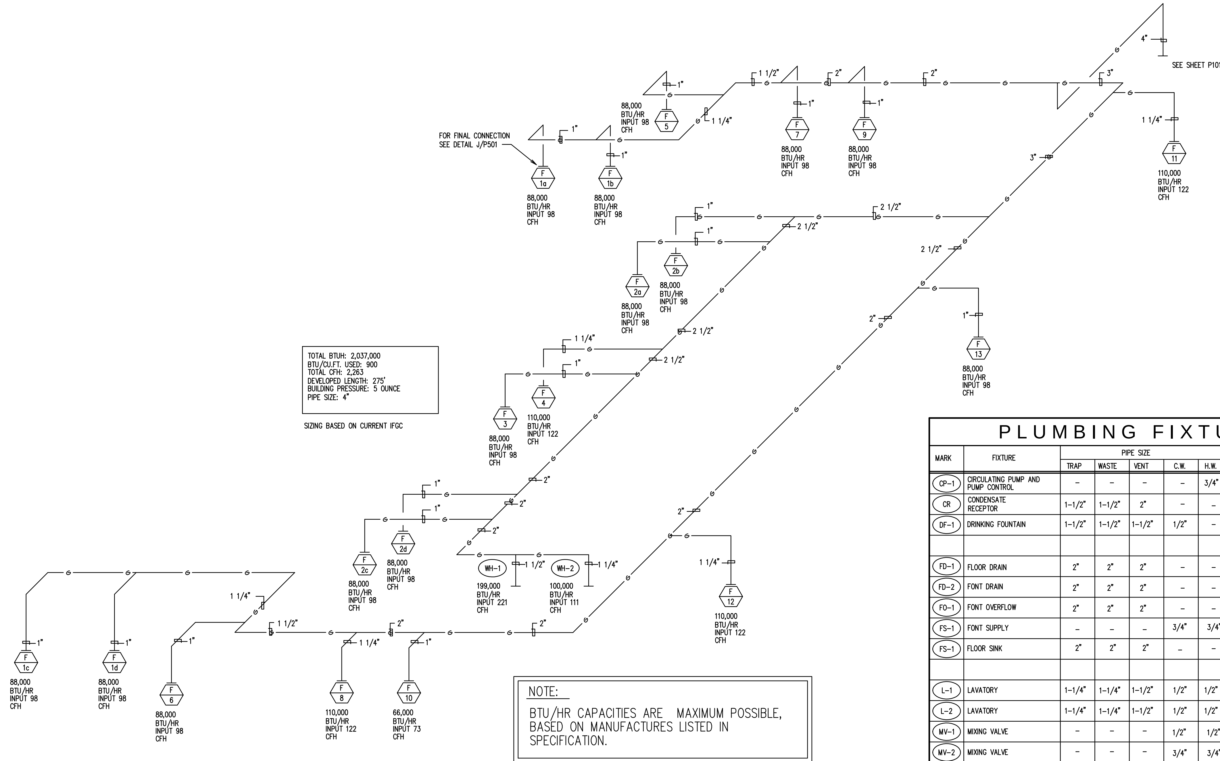
1 GAS PIPING SCHEME NOT TO SCALE
