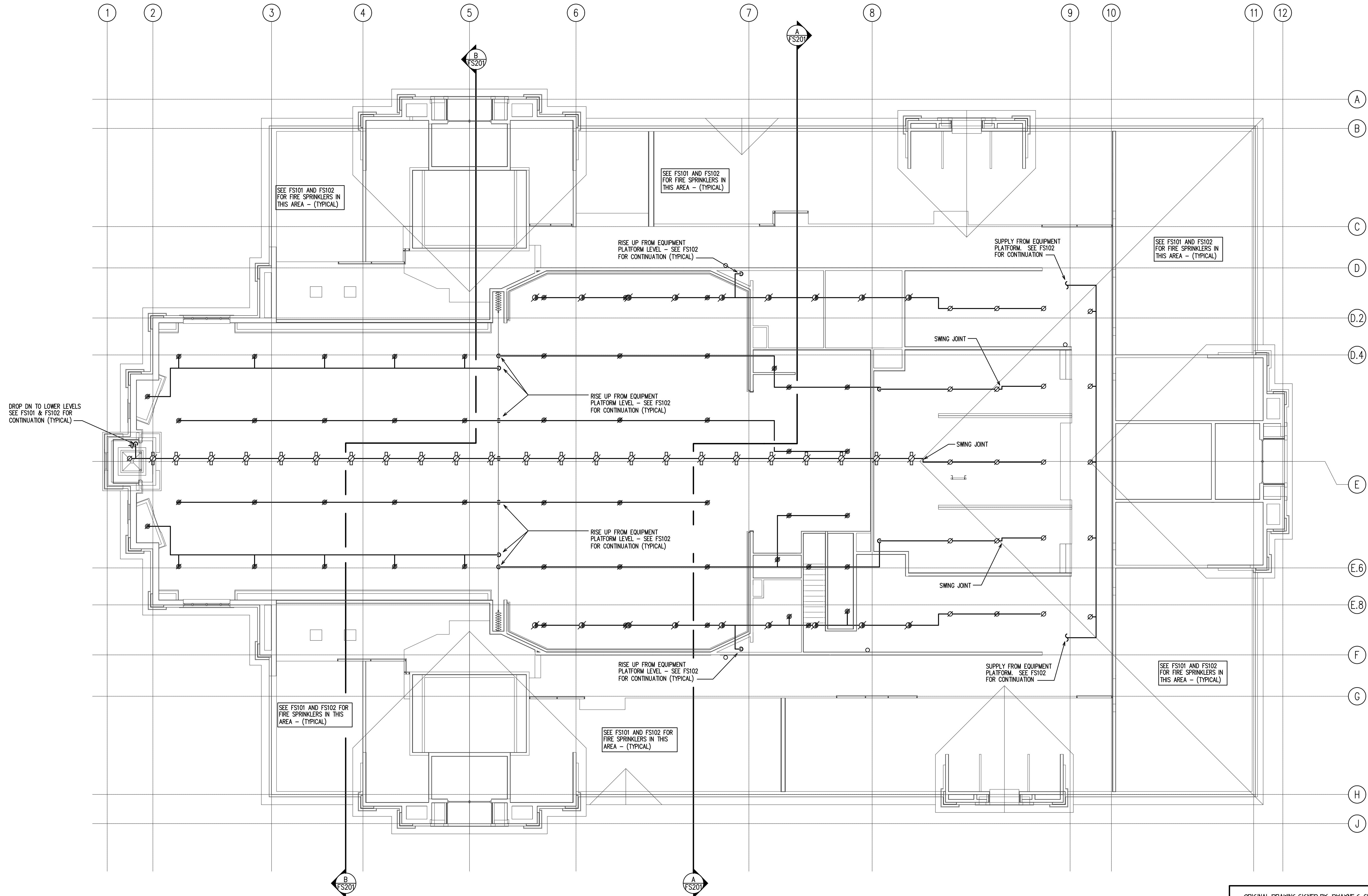
3 ATTIC LEVEL FIRE SPRINKLER PLAN 1/8" = 1'-0"
