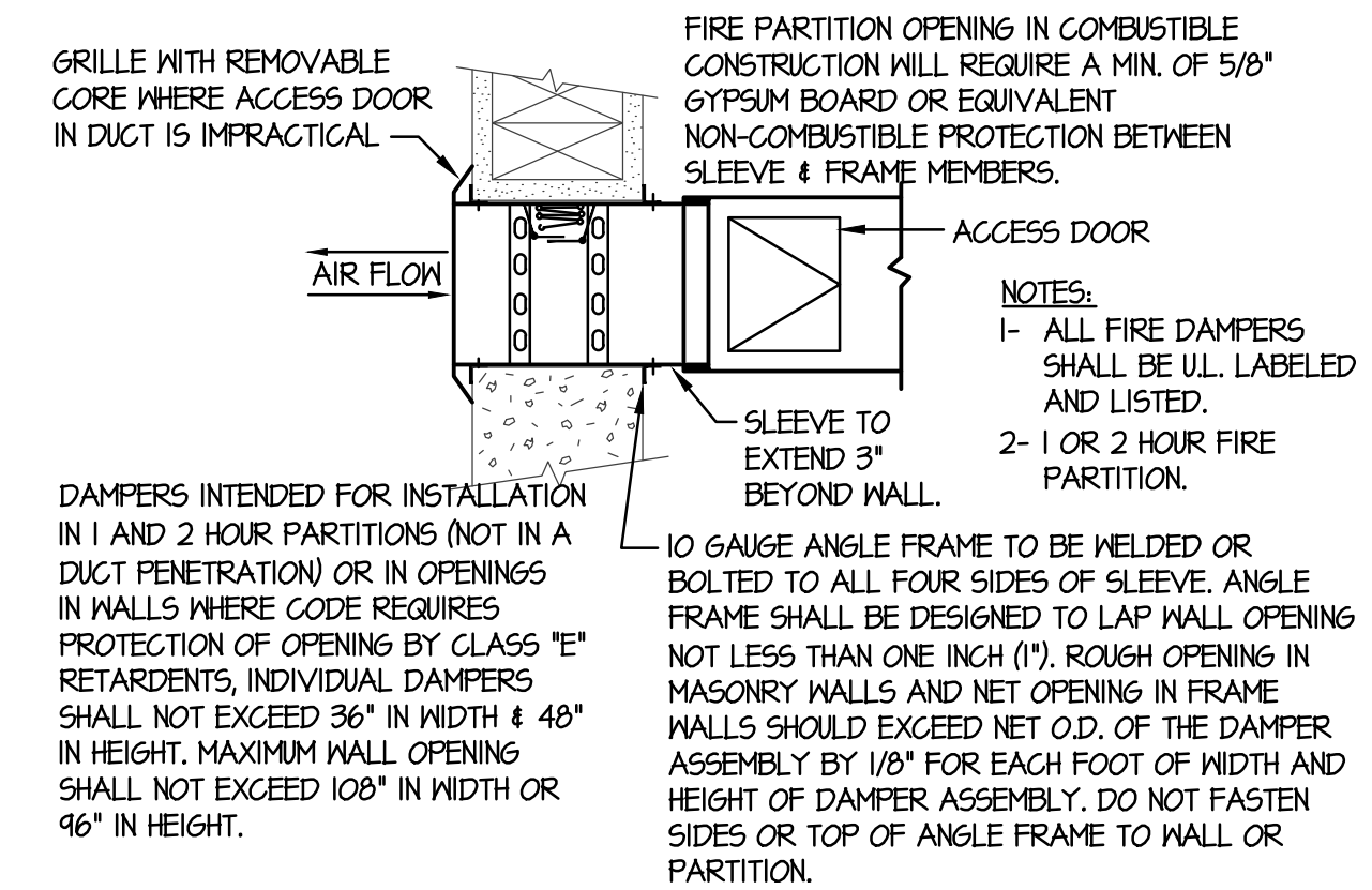
H SIDEWALL FIRE DAMPER DETAIL NO SCALE
