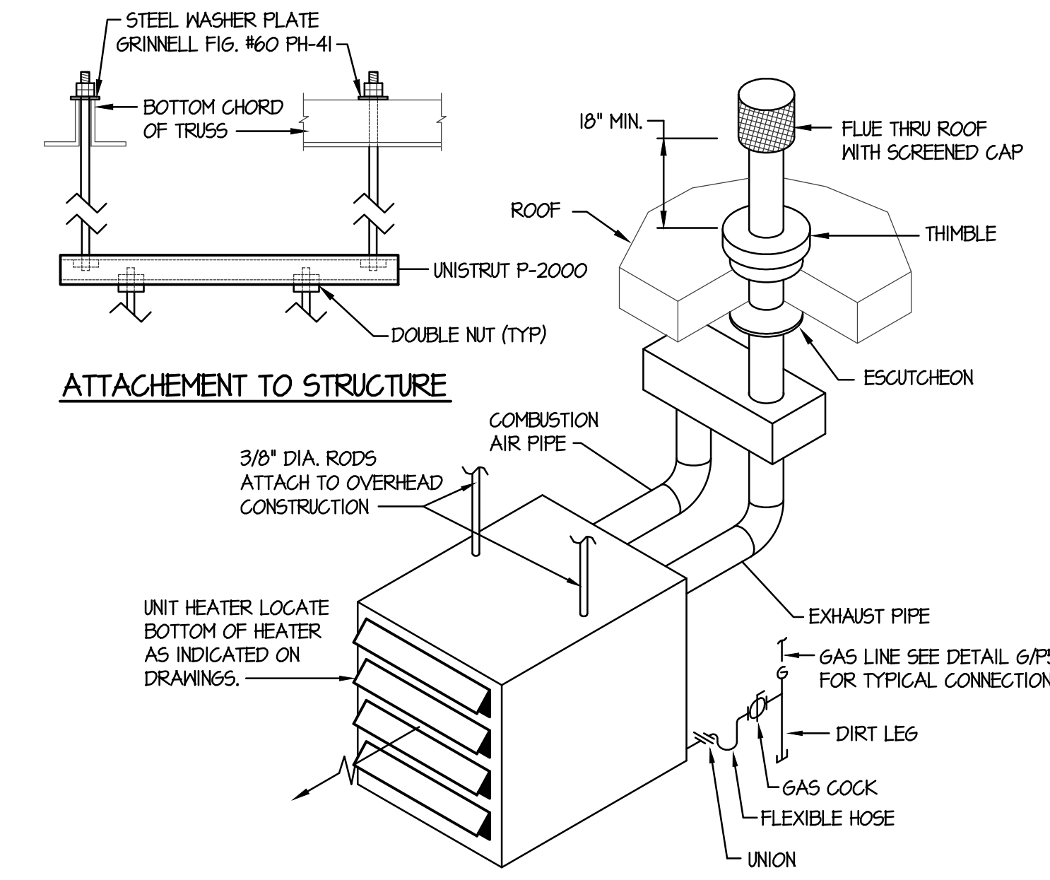
F SEPARATED COMBUSTION GAS FIRED UNIT HEATER DETAIL NO SCALE
