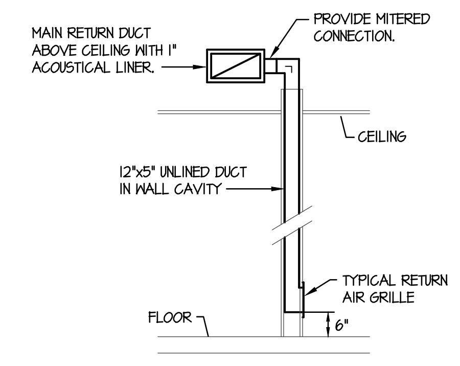
D RETURN AIR GRILLE DETAIL NO SCALE
