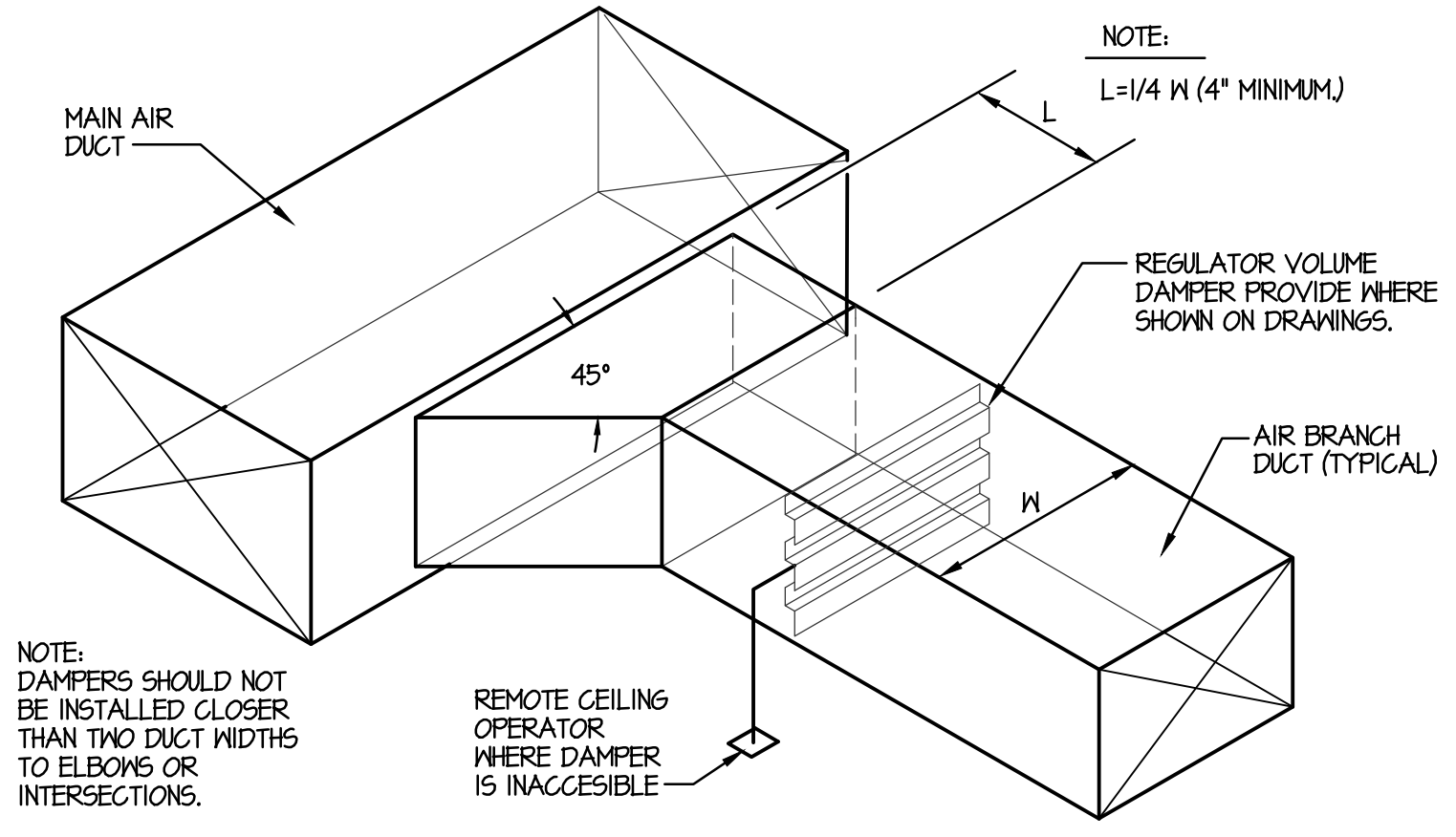
B SUPPLY OR RETURN AIR DUCT BRANCH CONNECTION DETAIL SCALE: NONE
