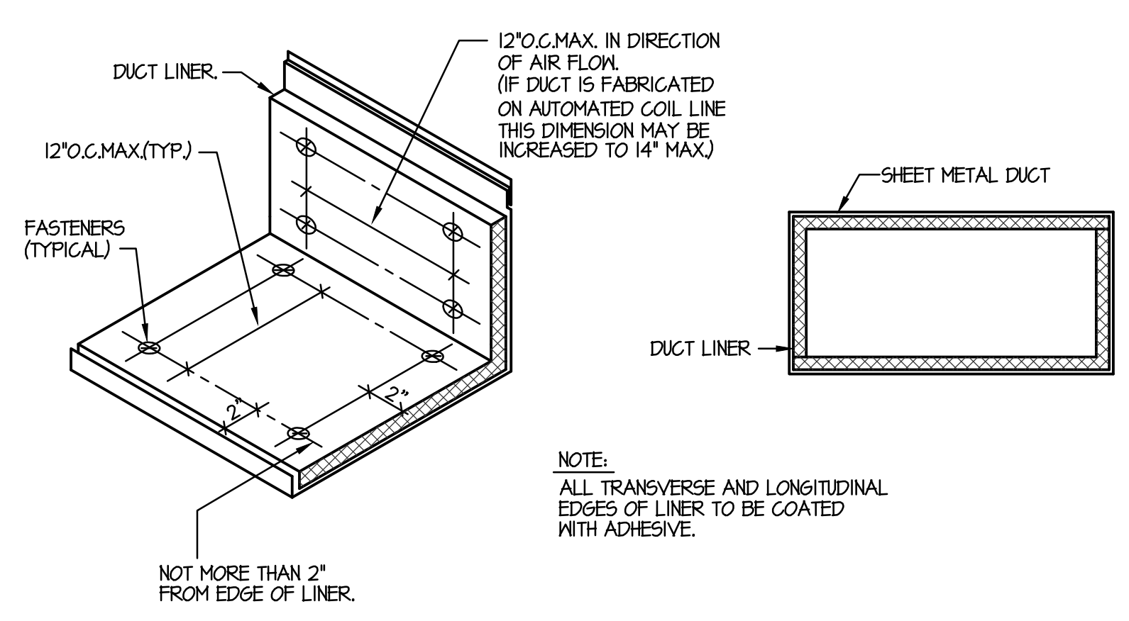
A DUCT LINER DETAIL SCALE: NONE
