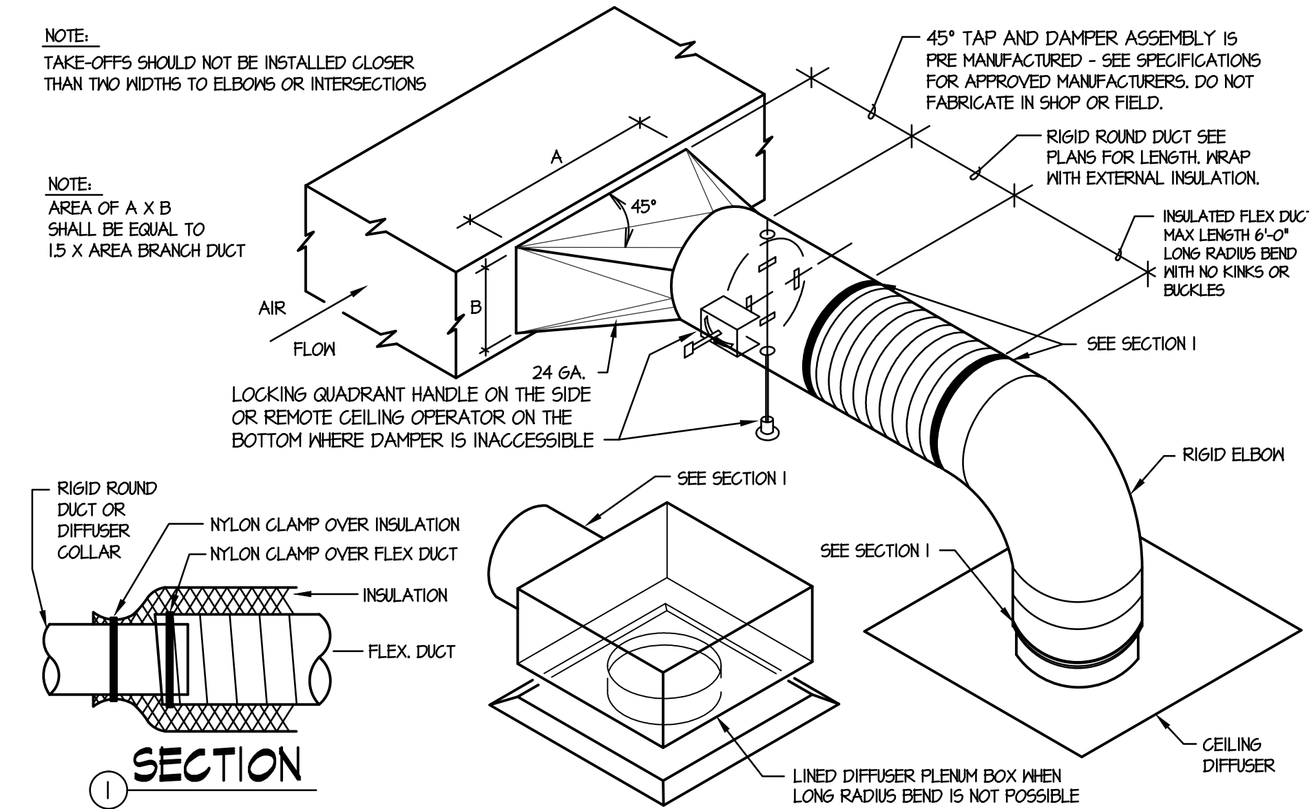
E SQUARE TO ROUND TAKE-OFF DETAILS NO SCALE
