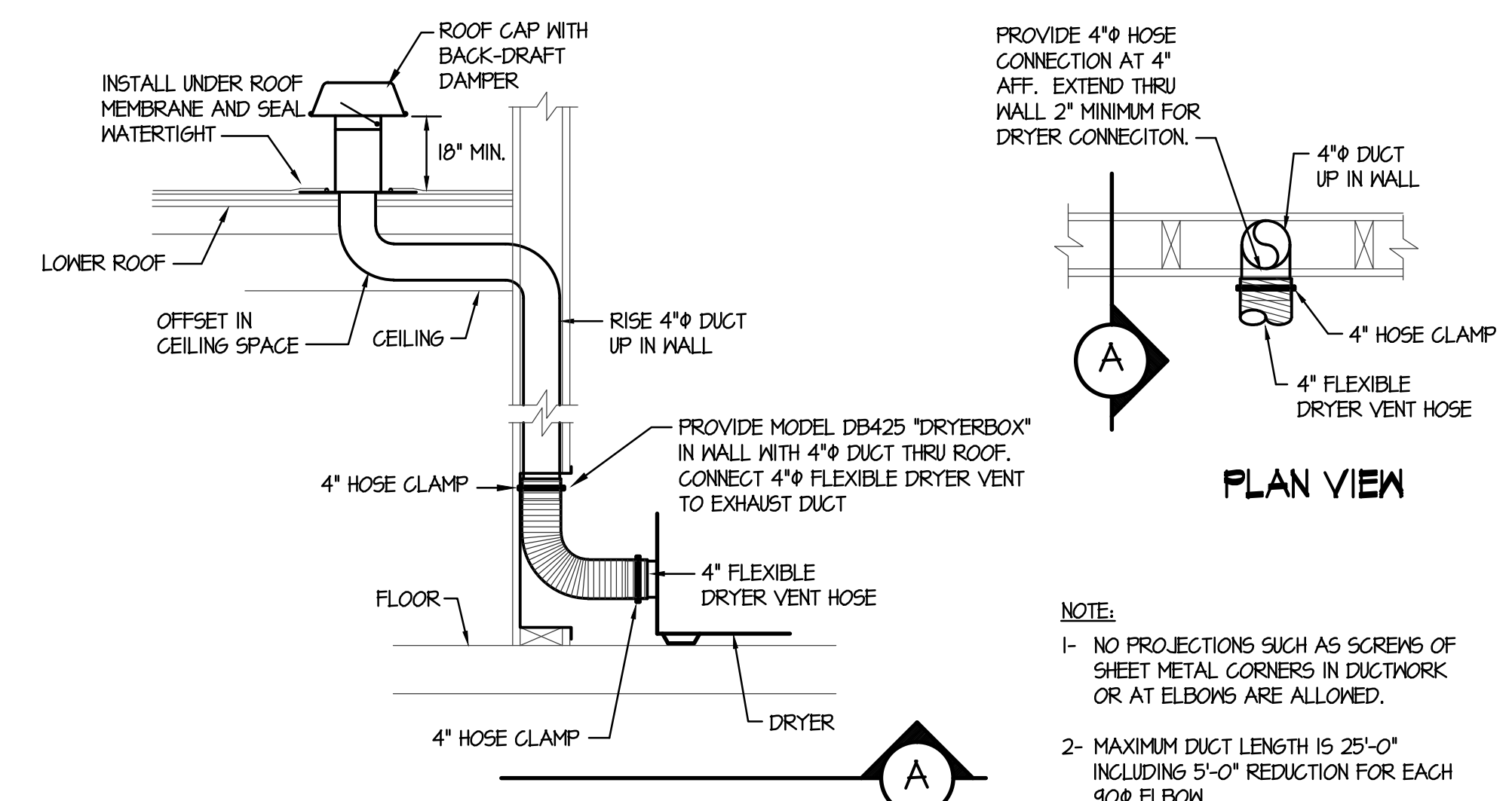
J DRYER VENT DETAIL NO SCALE
