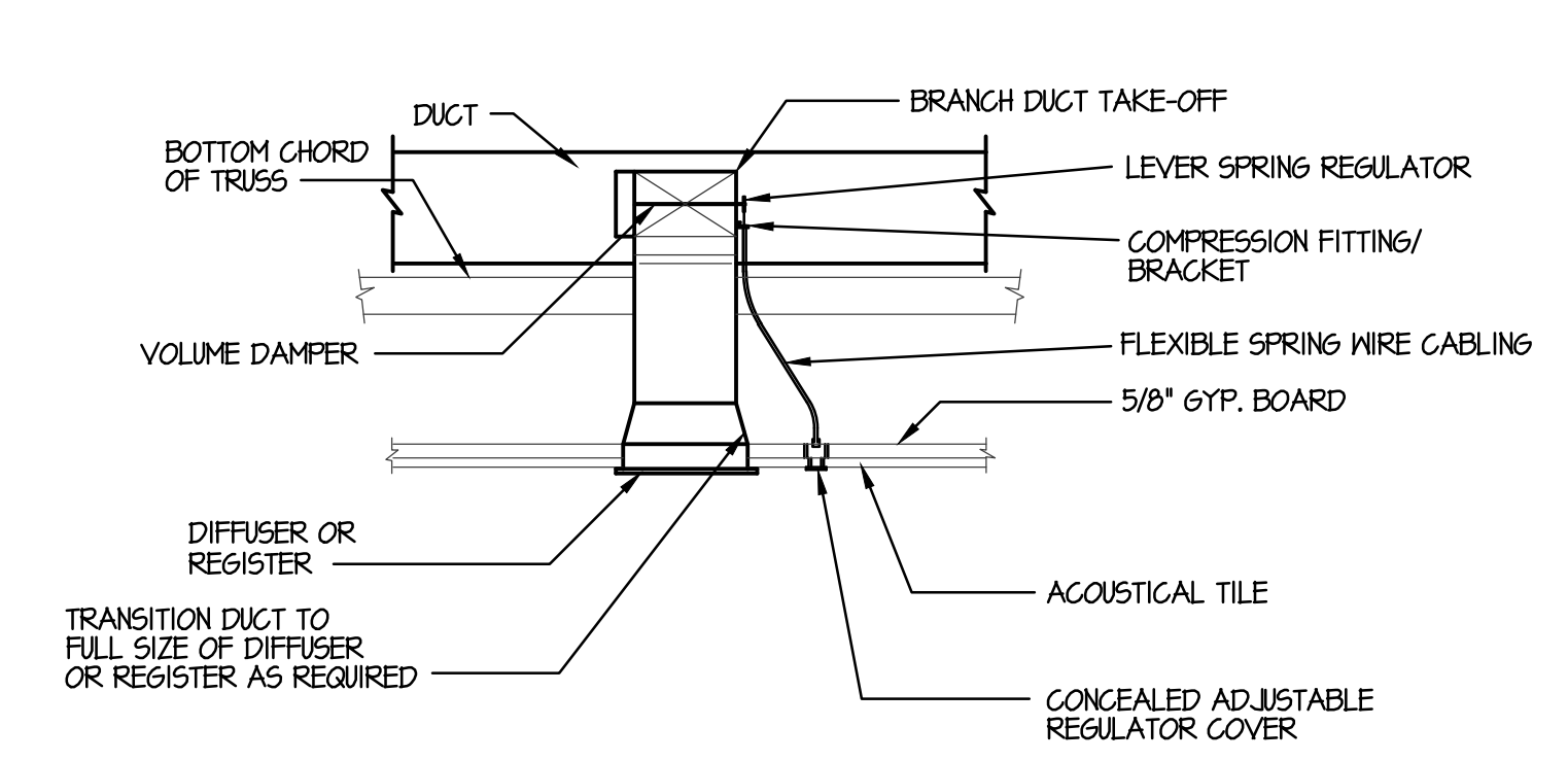
C TYPICAL REMOTE OPERATED DAMPER NOT TO SCALE
