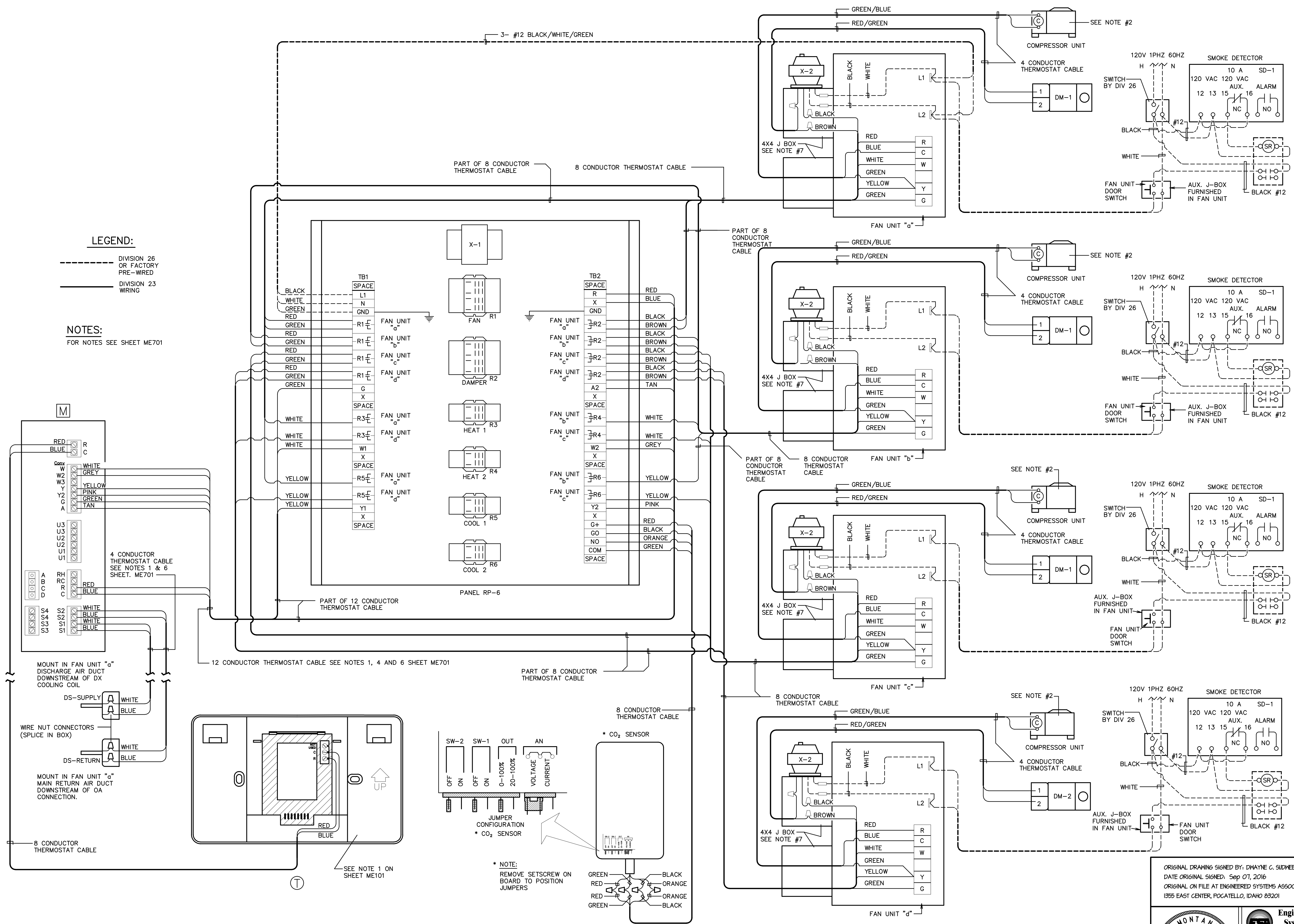
CHAPEL WIRING DIAGRAM SYSTEM: F-8
